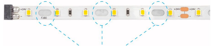
Bending gaps after every 2 LEDs (1.31")
